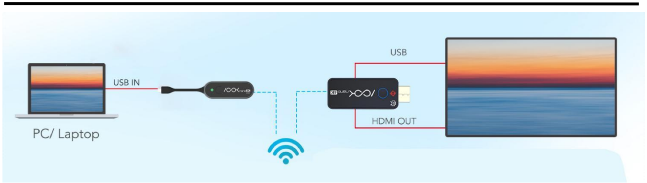
ASK nano 4K (USB-C) System Connection Diagram 1
