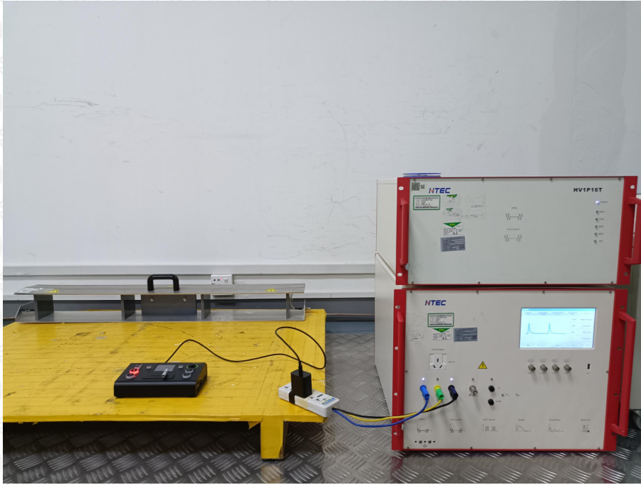
Figure 5: SURGE、DIP&EFT Test Setup
