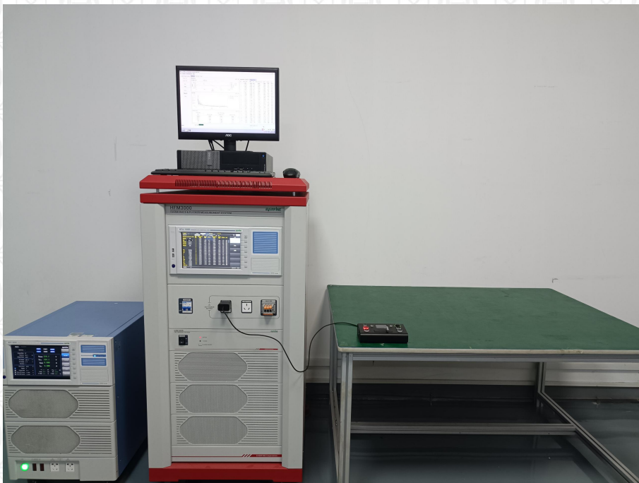
Figure 6: Harmonic & Flicker Test Setup
