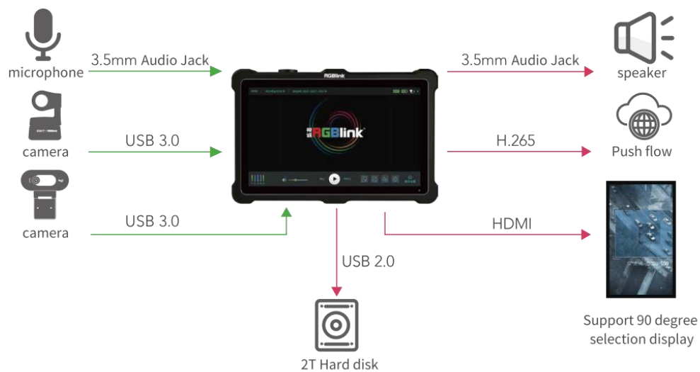
SYSTEM CONNECTION
