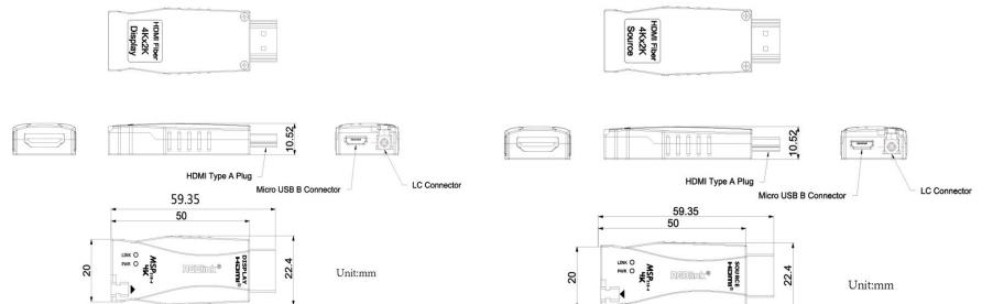
MSP 318-4 Transmitter
