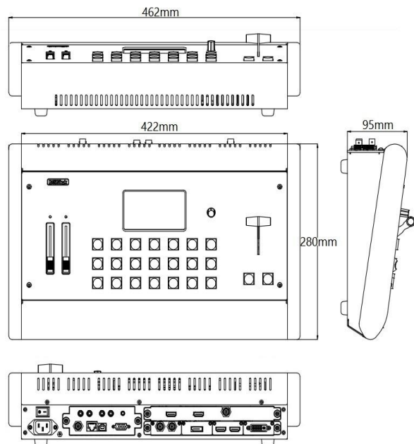
M1 with optional fitted wings/sides
