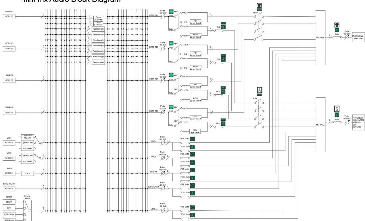
mini-mx Audio Block Diagram
