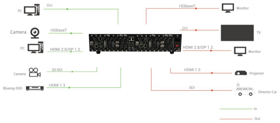
FLEX 9(MINI) Connection Diagram
